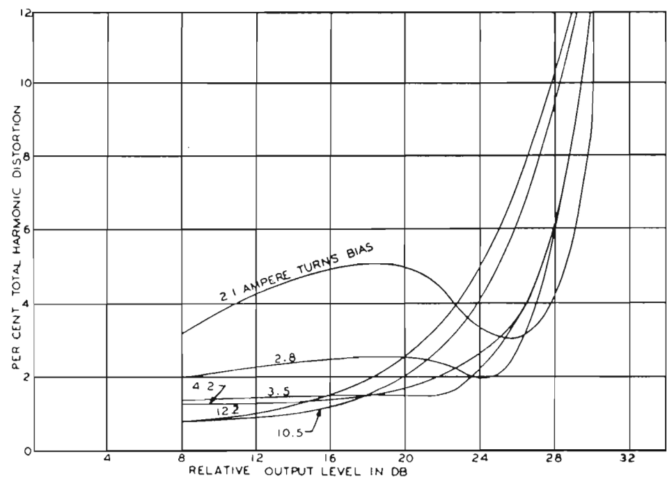
Fig. 3. Distortion versus reproducing level (duPont SW4 tape).
