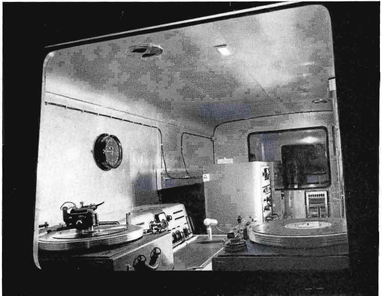
FIG. 2. This view through rear window of the mobile unit shows the location of the transcription recorders, the 76B-5 Console, and the transmitter and the monitoring racks.
