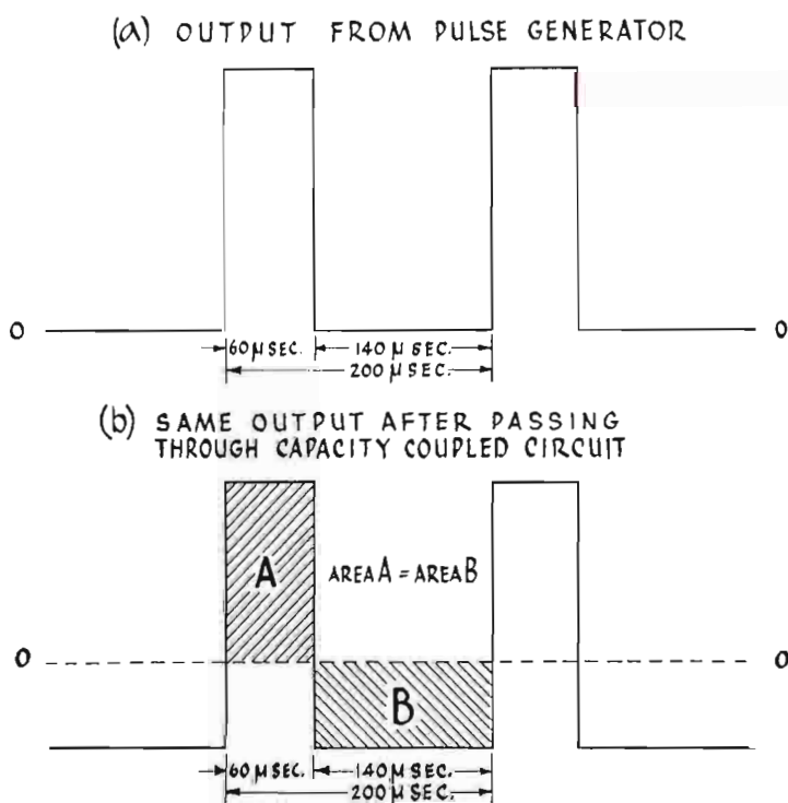
FIG. 12. Averaging effect of capacity-coupled circuit upon positive pulse.
