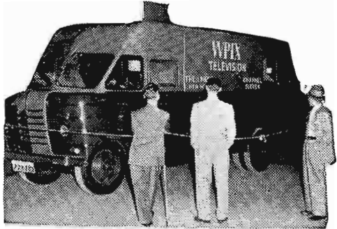
Television Studio-on-Wheels. This special RCA TV field truck is handling the track sound-and-picture pick-up between Roosevelt Raceway grandstand and WPIX in New York City. All RCA-equipped, it is designed to carry everything needed to operate up to 3 cameras in the field.
