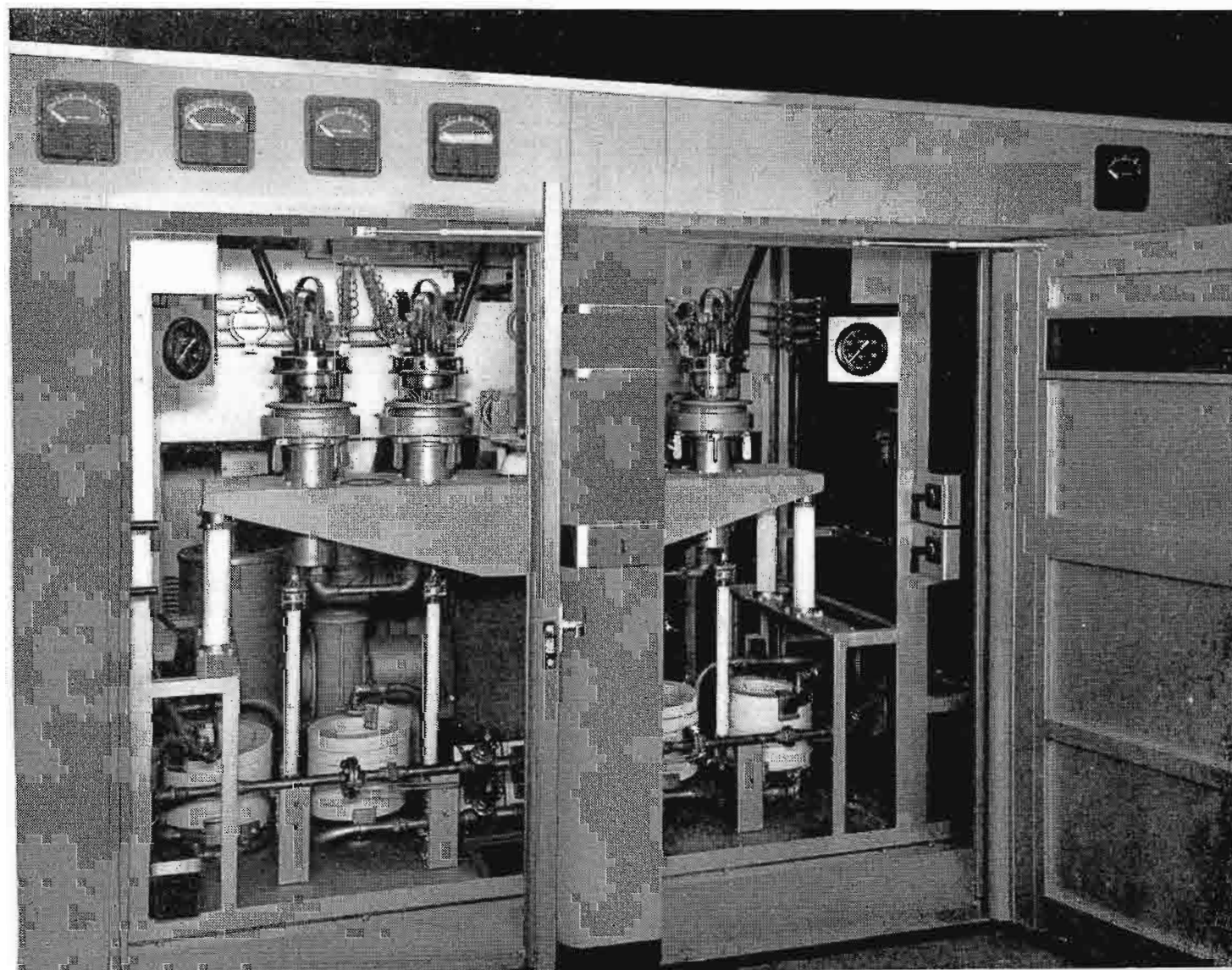
FIG. 10 (below). In this view doors to the 150 KW power amplifier are opened to illustrate the assembly of the four 9C21 power tubes on a single base plate.
