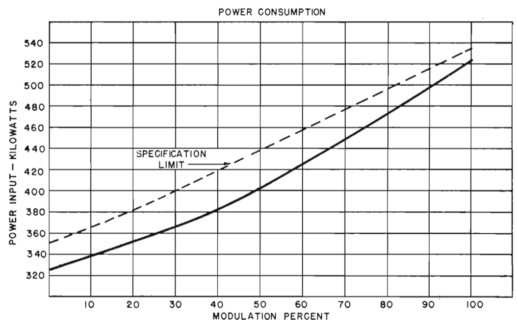
FIG. 16 (at right). Curve of 150 KW transmitter power input vs. modulation percent compared to specification limits.
