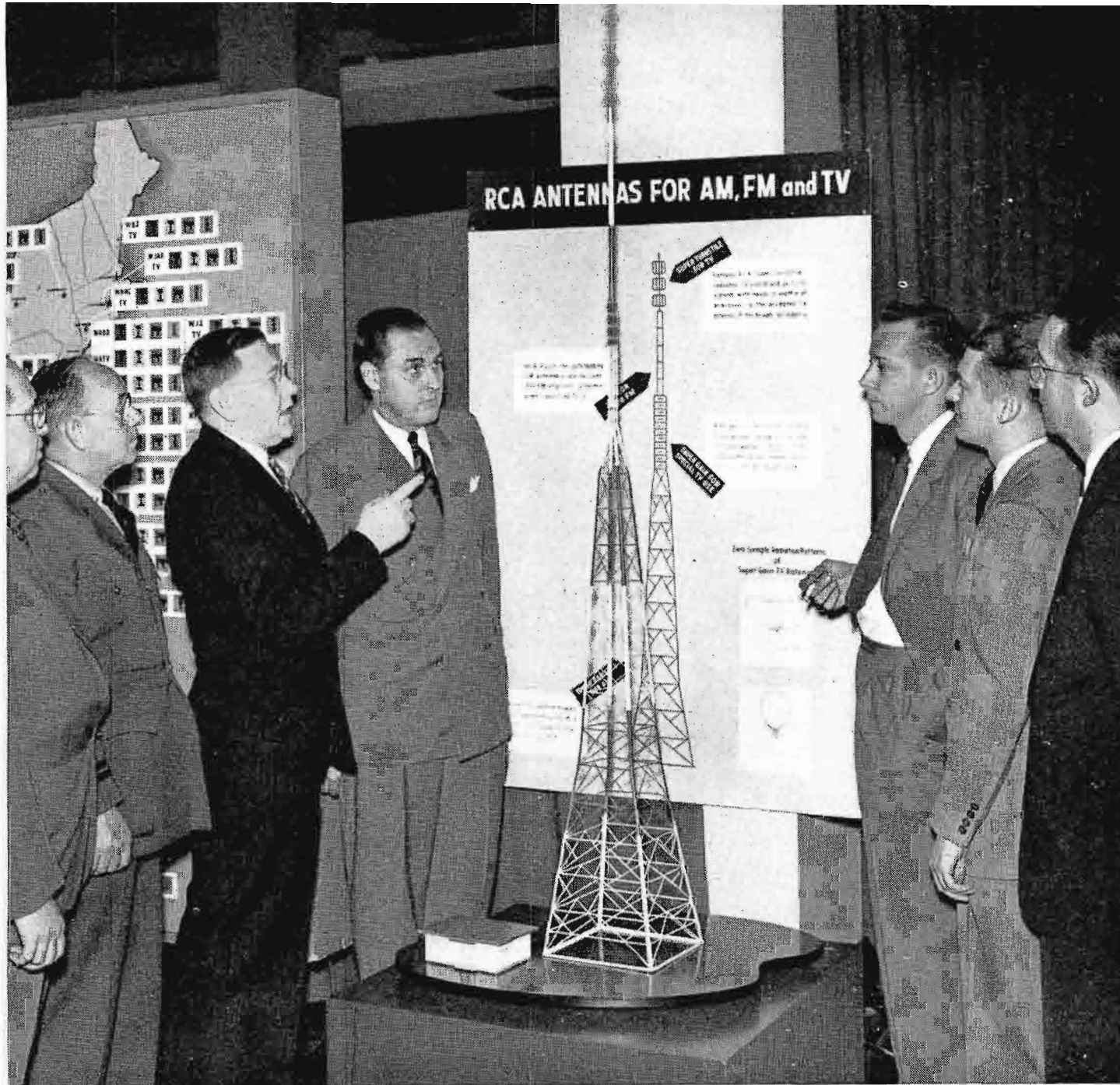
FIG. 4. The unique antenna system represented by the model shown above can perform six different services, E. S. Clammer told broadcasters. Two TV programs, three FM programs, and one AM program can be broadcast from the actual tower simultaneously. The model tower includes a Supergain antenna, a four-section Pylon, and a three-section Super-Turnstile.
