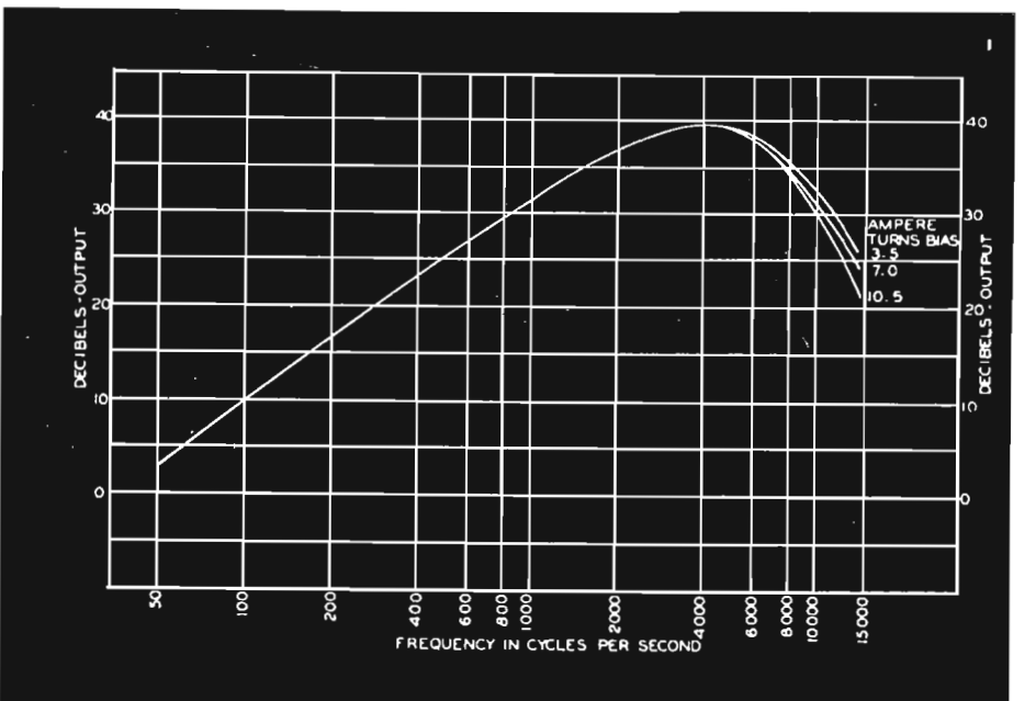
FIG. 13. Frequency Response, Minnesota Mining Type RR tape.
