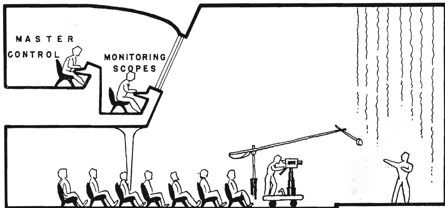
FIG. 2. Section through studio and control room of the studio plan shown in Fig. 3 and Fig. 4 (following pages).
