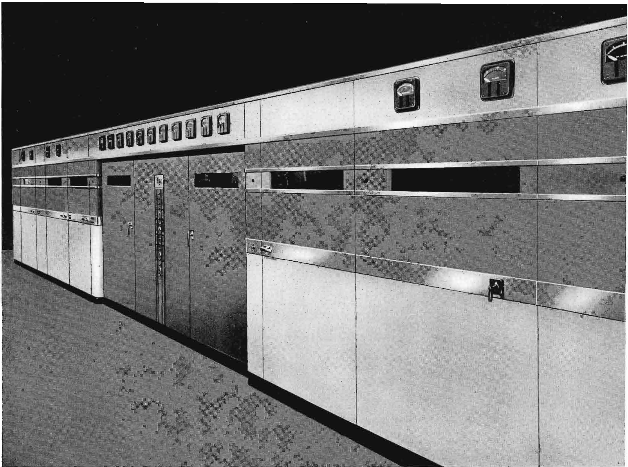
FIG. 2 (above). The final 150 KW transmitter design, as set up in "53" engineering building for final tests. All transmitter components are installed behind the unified front panel which presents a streamlined appearance. Radio Istanbul, powerful new voice of Turkey, is covering that country and the middle east with one of these new transmitters.
