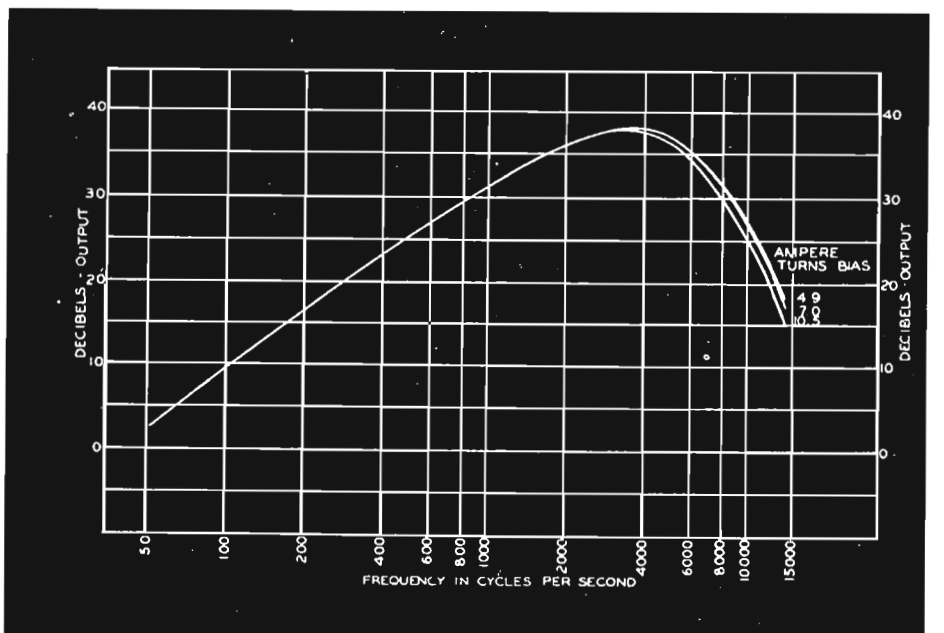
Fig. 12. Frequency Response, Minnesota Mining black-oxide plastic tape.
