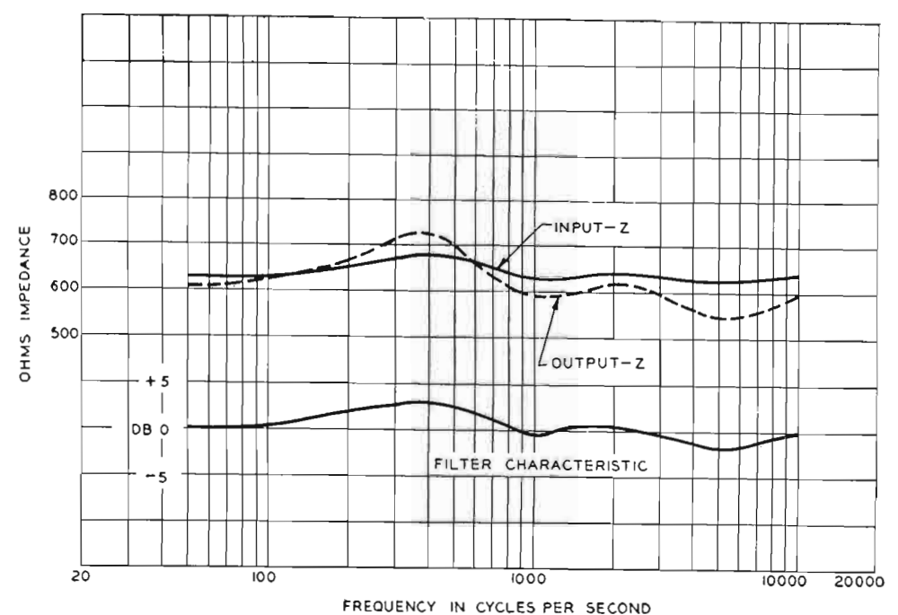
FIG. 5 (at right). Input and output impedance characteristics of the crossover filter for typical filter adjustments.
