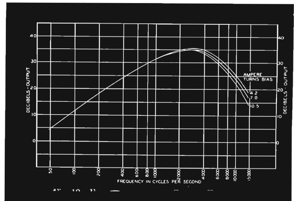
FIG. 10. Frequency Response, German Type C tape.
