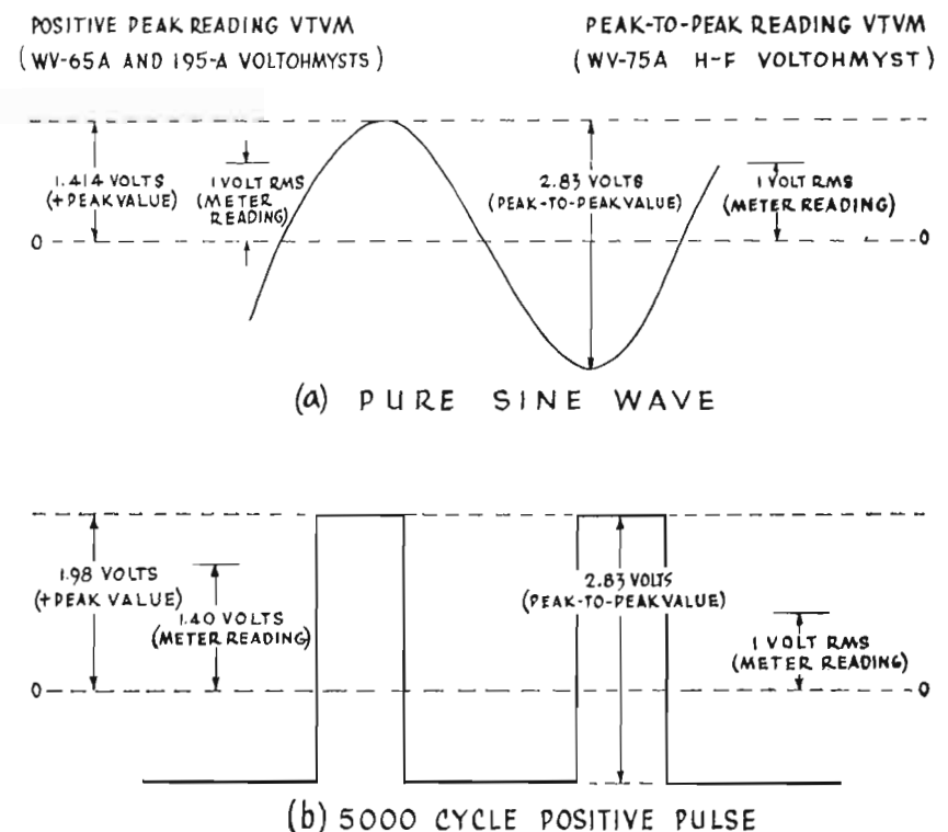
FIG. 13. How VTVM's measure sine waves and positive pulses.
