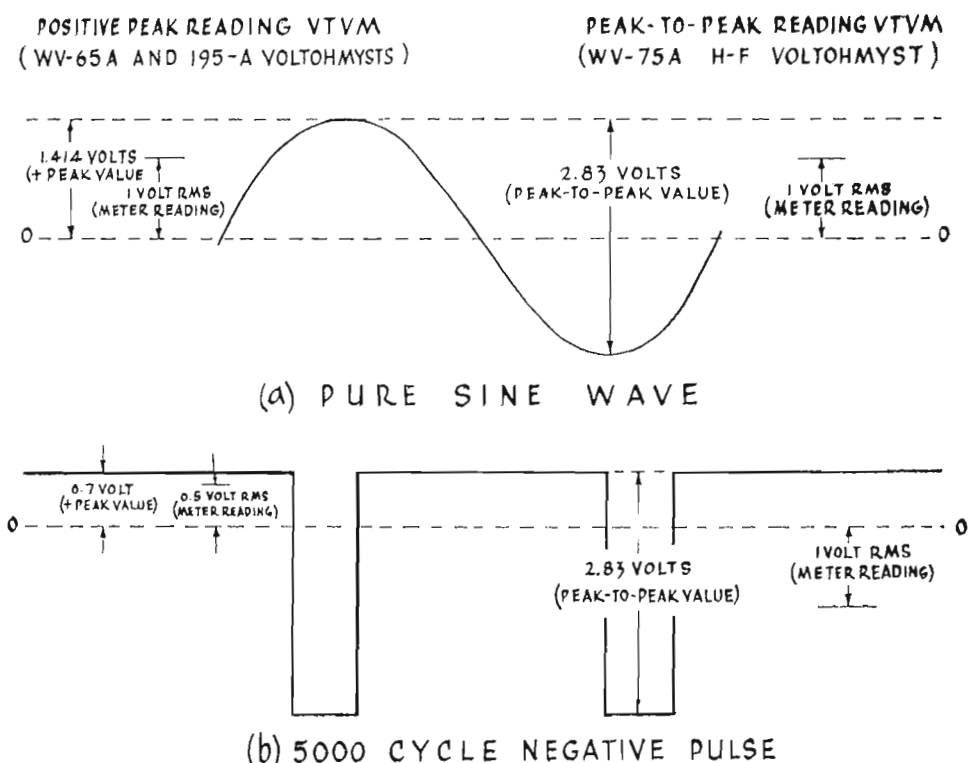
FIG. 17. How VTVM's measure sine waves and negative pulses.
