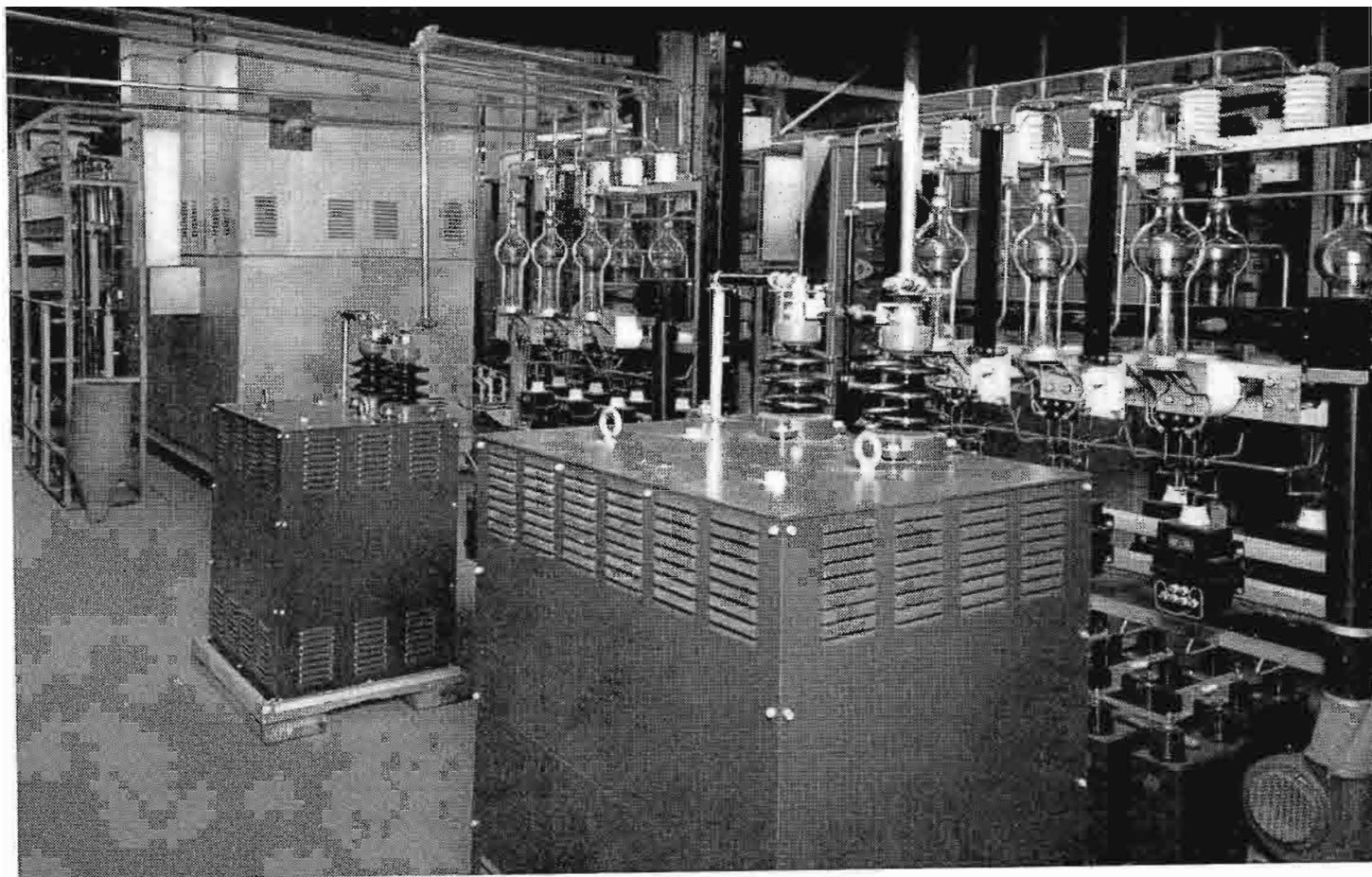
FIG. 11 (above). View of the 11.5 KV and 14 KV rectifier assemblies with associated filter reactors also visible.
