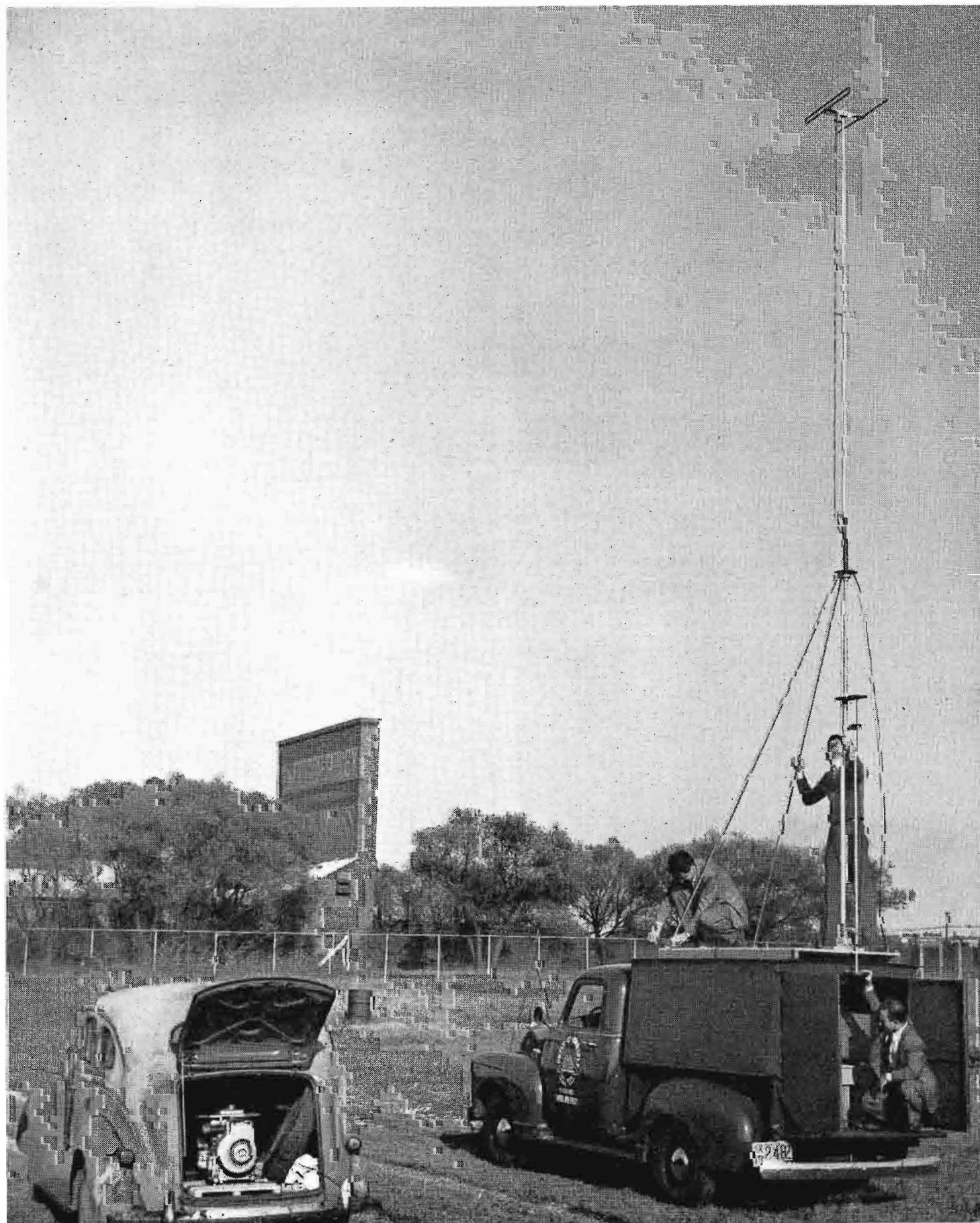
FIG. 2. A 750-watt gasoline powered generator supplied all the power necessary for the receiving and calibrating equipment located in the mobile monitoring truck.
