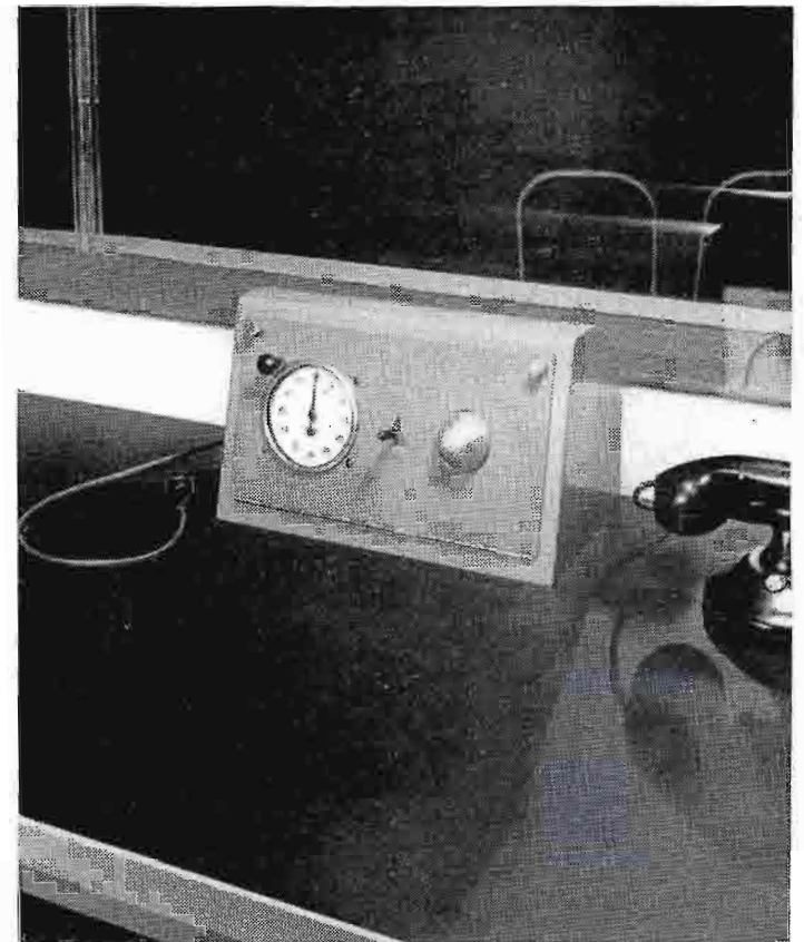
FIG. 8. The program directors' or producers' turret and controls shown here are located adjacent to studio "A" and "B" consoles and consist of talkback microphone, operate switch and timer.
