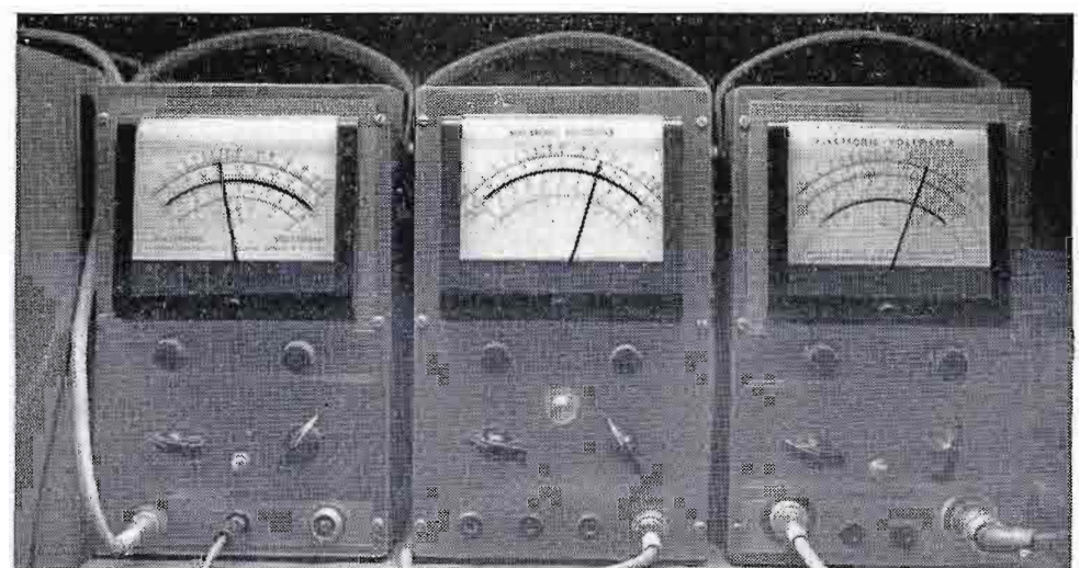
FIG. 6. Type 195-A 2.2 volts (rms) Type WV-65A (with Crystal Probe) 2.2 volts (rms) Type WV-75A 2.15 volts (rms)
