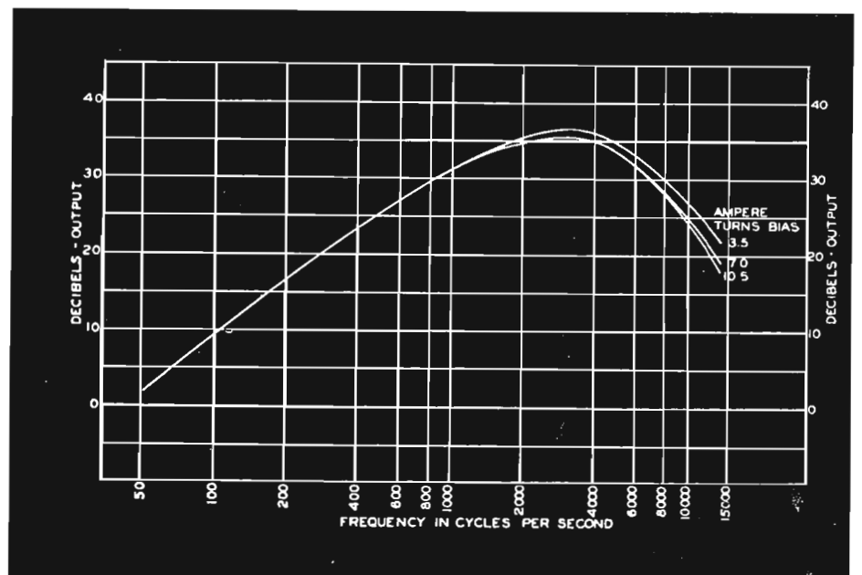
FIG. 11. Frequency Response, duPont SW4 tape.
