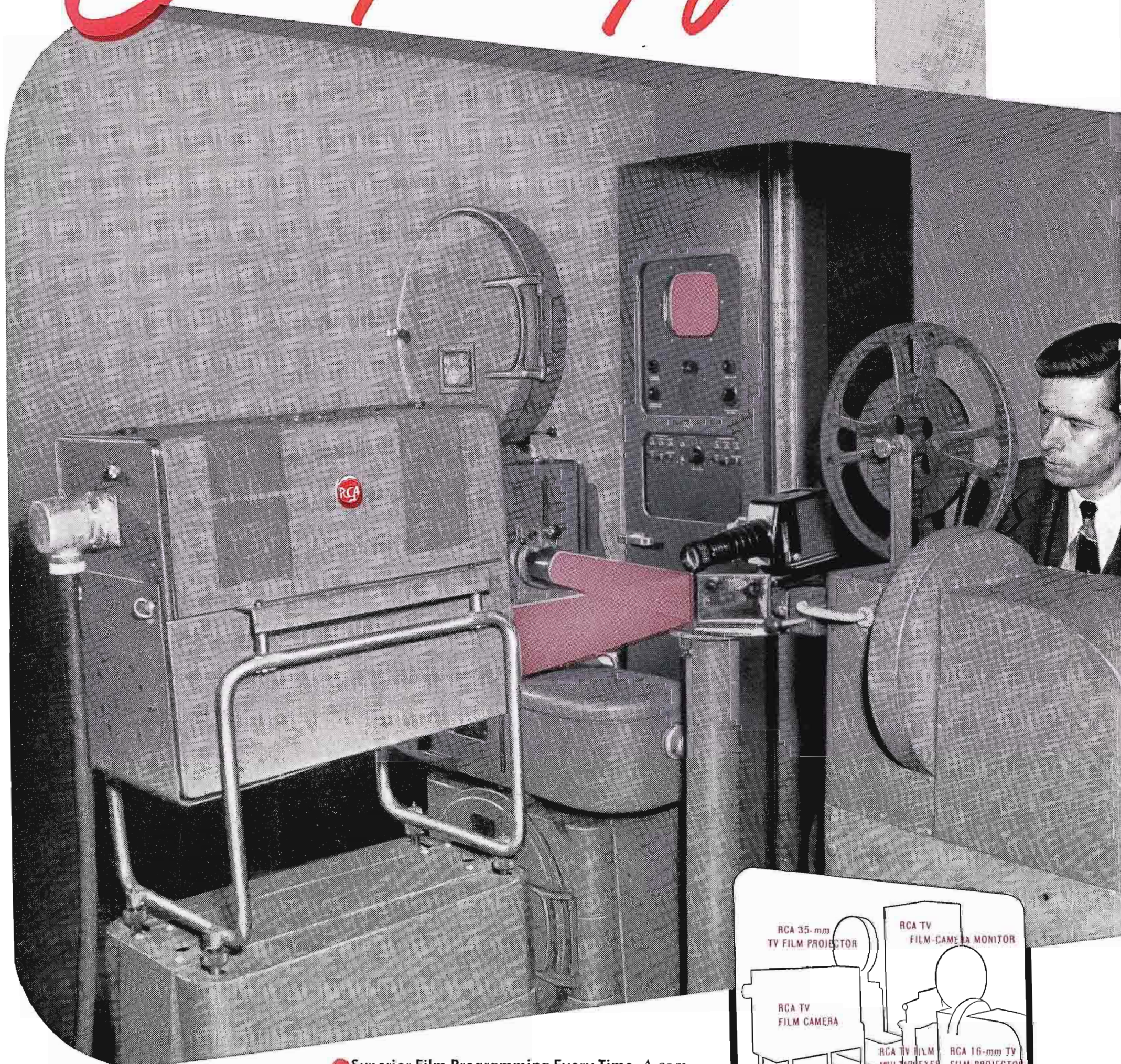
● Superior Film Programming Every Time. A completely equipped TV film-projection room by RCA —one of nearly 10 different combinations now being delivered to more than 50 television stations throughout the country.
