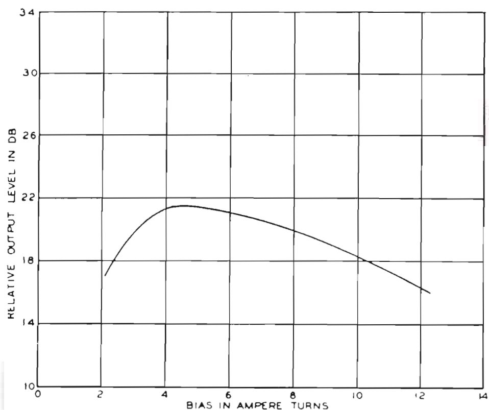
FIG. 9. Output level versus bias for Minnesota Mining Type RR tape.
