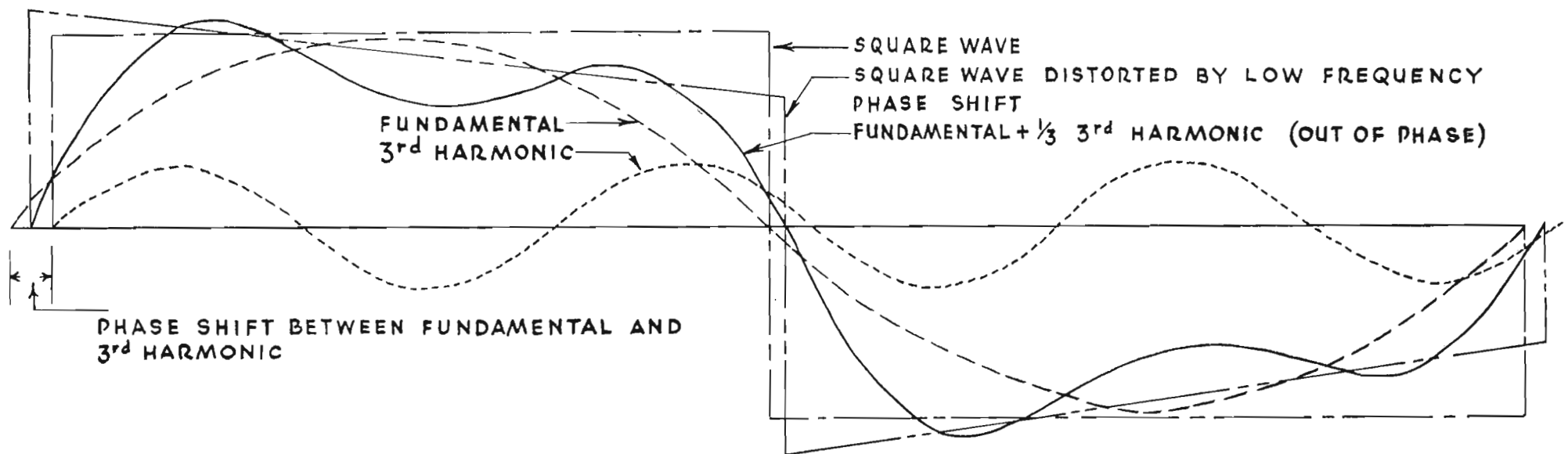
FIG. 21. This figure shows the effect of phase shift. The fundamental frequency is shown slightly out of phase with its third harmonic. When the fundamental and shifted harmonic are added, the resulting wave has a tilt. Similarly, a square wave which has some of its components shifted in phase will show a tilt.
