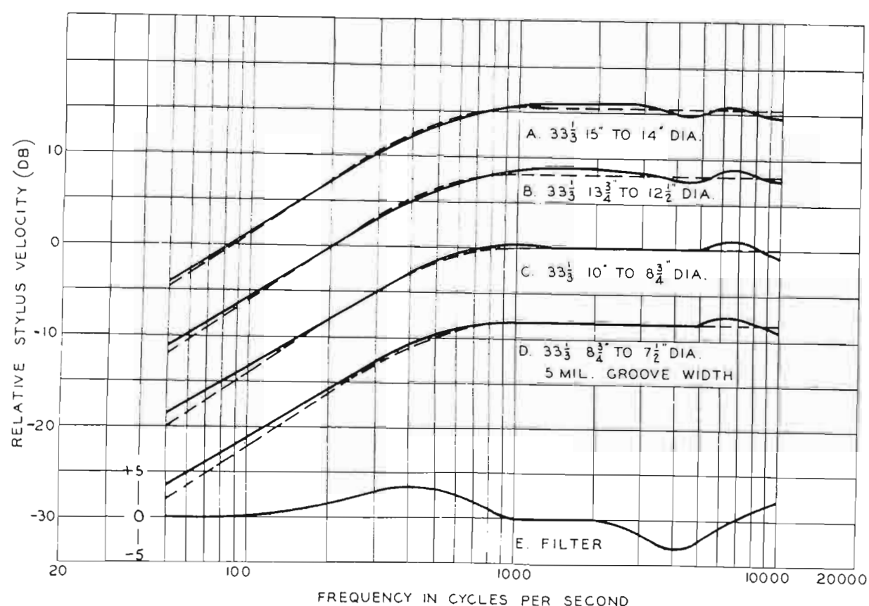
FIG. 8. Response characteristic at different recording diameters and 33 \frac{1}{3} rpm. Note how little change occurs between outside and inside of the disk.
